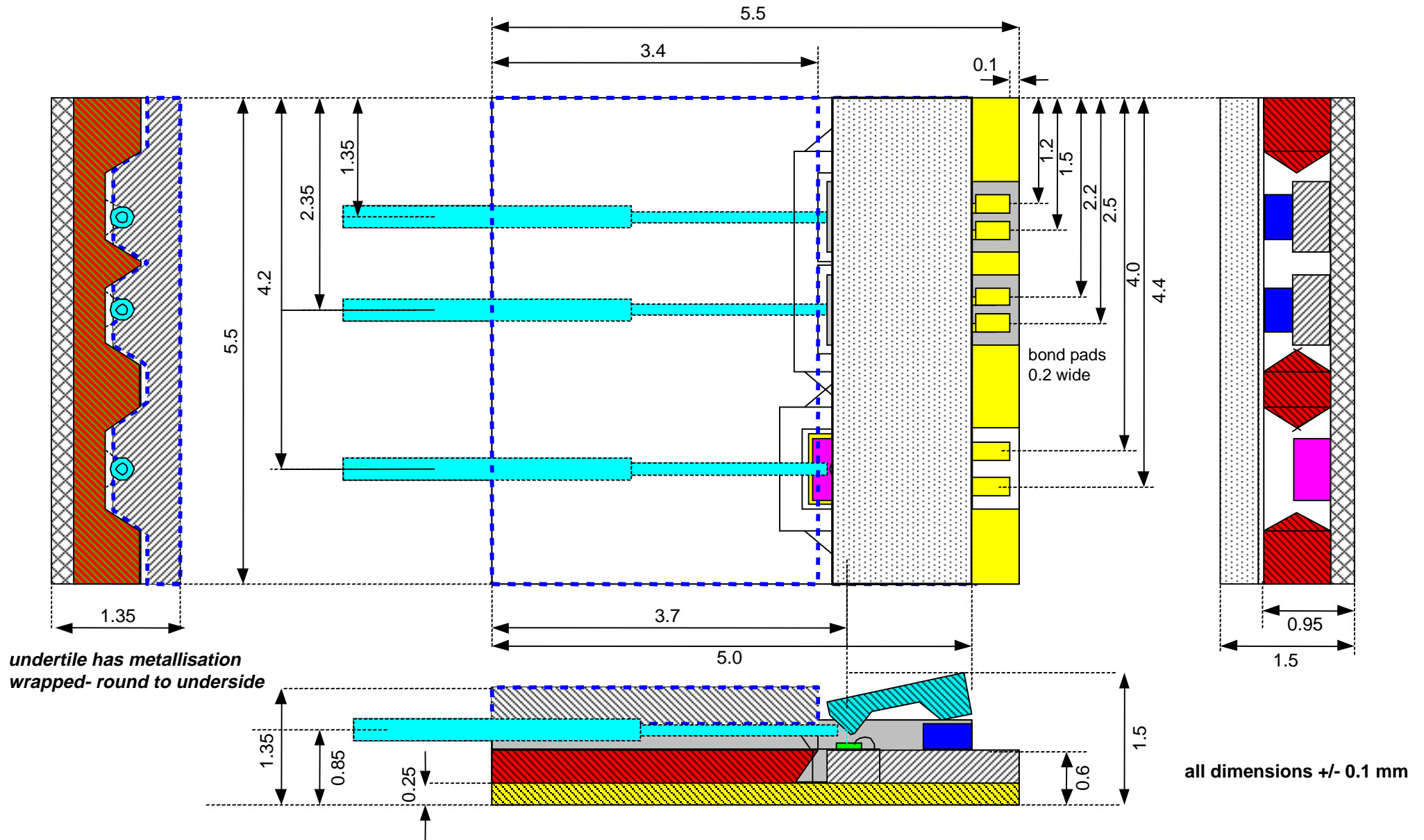
Silicon packaged VCSEL-PIN unit - schematic showing proposed key dimensions prepared by J. Hall 25.3.99 - Marconi Materials Technology, Caswell
