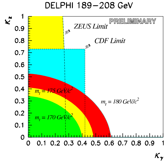
Fig. 3. Exclusion regions in the LEP convention at 95% C.L. in the \kappa_\gamma - \kappa_Z plane from DELPHI, CDF and ZEUS. The ZEUS limit has been converted to take into account a factor \sqrt{2} between the LEP convention and that used for Fig. 2.
