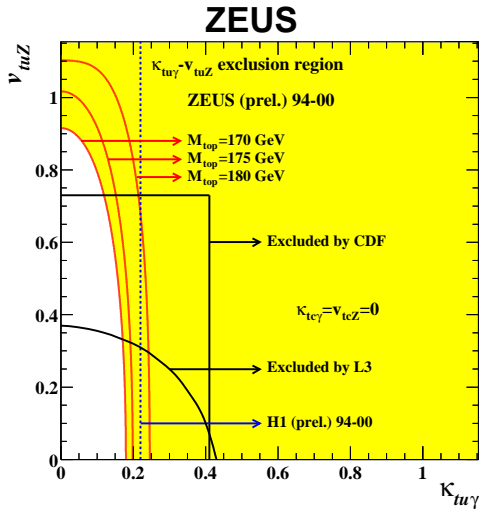
Fig. 2. Exclusion regions at 95% C.L. in the \kappa_{t\bar{u}\gamma} - \nu_{t\bar{u}Z} -plane from L3, CDF, H1 and ZEUS.
