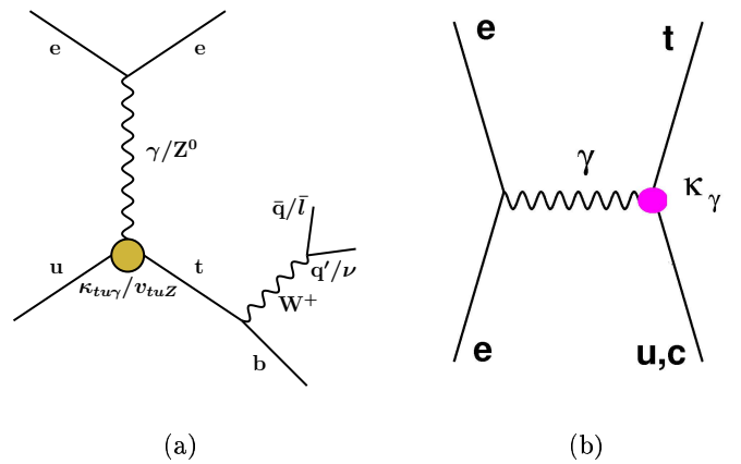
Fig. 1. Feynman diagrams for single-top production via FCNC transitions at (a) HERA and (b) LEP.
