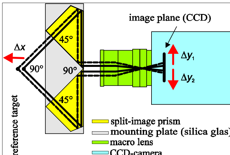
Figure 5: optical 3D-sensor
