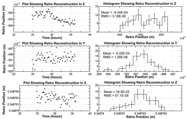
Figure 13: Reference marker reconstruction over a 14 hour period along with the histograms of that data
