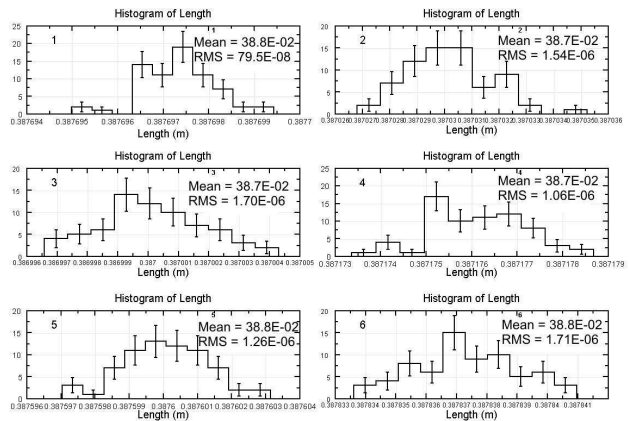
Figure 12: Histogram of lengths measured by external FSI system over a 14 hour period
