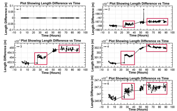
Figure 16: The lengths measured by the internal FSI on car 3 with the lengths of line 1 subtracted during a 90 hour period. Regions of interest are marked
