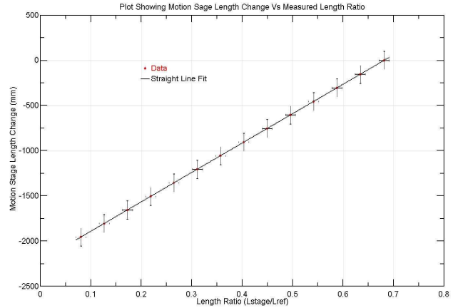
Figure 8: Data from length calibration experiment with fit results. Note: error bars are magnified by 10000
