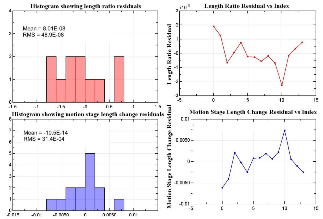
Figure 9: The residues of the fit and data from figure 8
