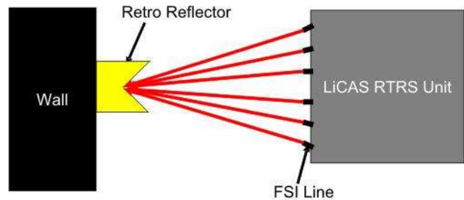
Figure 4: Sketch of External FSI System
