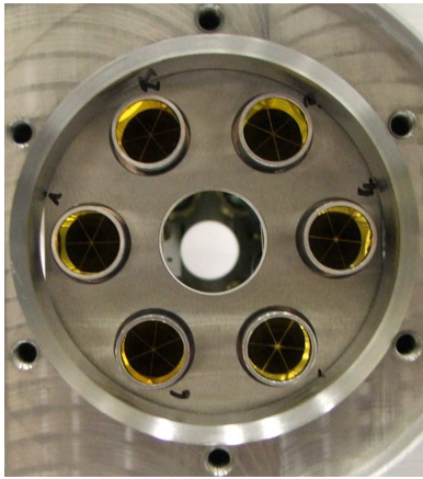
Figure 6: Photo of the mounted internal FSI retro reflectors
