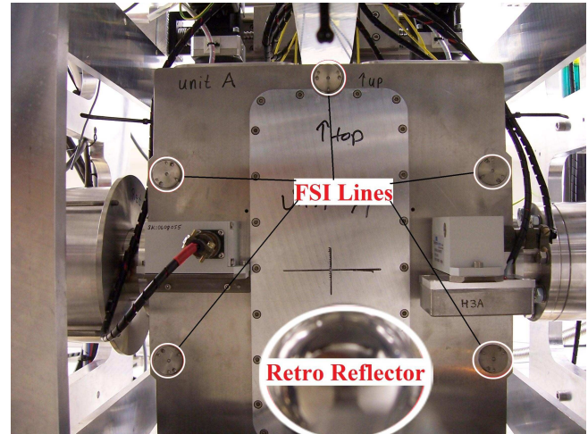
Figure 3: Photo of a LiCAS unit installed observing a retro reflector
