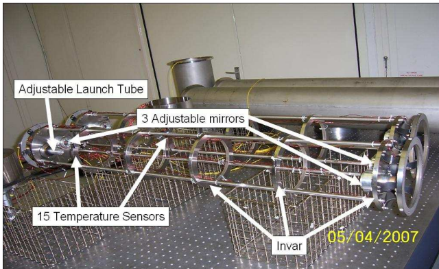
Figure 1: Photo of the two LiCAS reference interferometers under construction in Oxford
