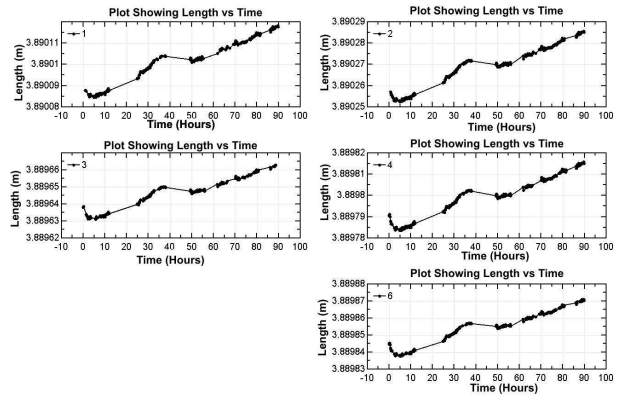
Figure 15: The lengths measured by the internal FSI on car 3 during a 90 hour period
