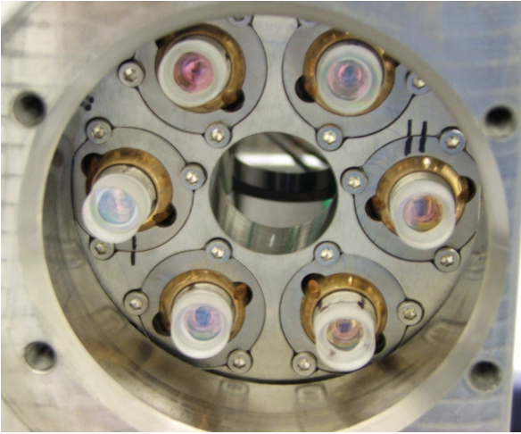
Figure 5: Photo of the mounted internal FSI launch optics
