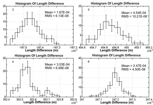
Figure 17: Histogram of the lengths measured by the internal FSI on car 3 with the lengths of line 1 subtracted during a 30 hour period
