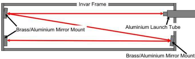
Figure 2: Sketch of a LiCAS Reference Interferometer
