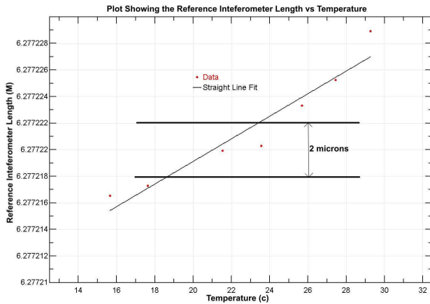
Figure 10: Data From the first pass of the thermal calibration of one of the LiCAS reference interferometers
