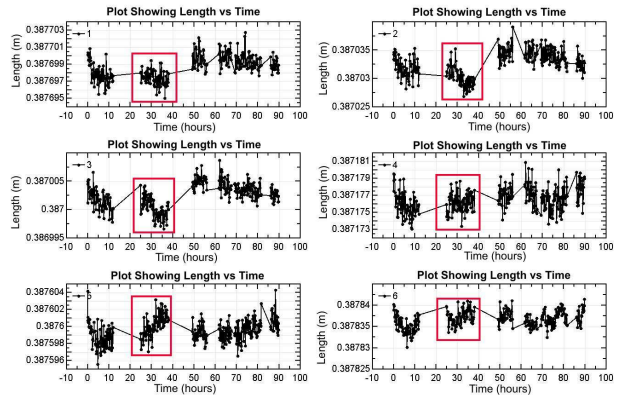
Figure 11: Lengths measured by external FSI system over a 90 hour period. Regions of interest are marked
