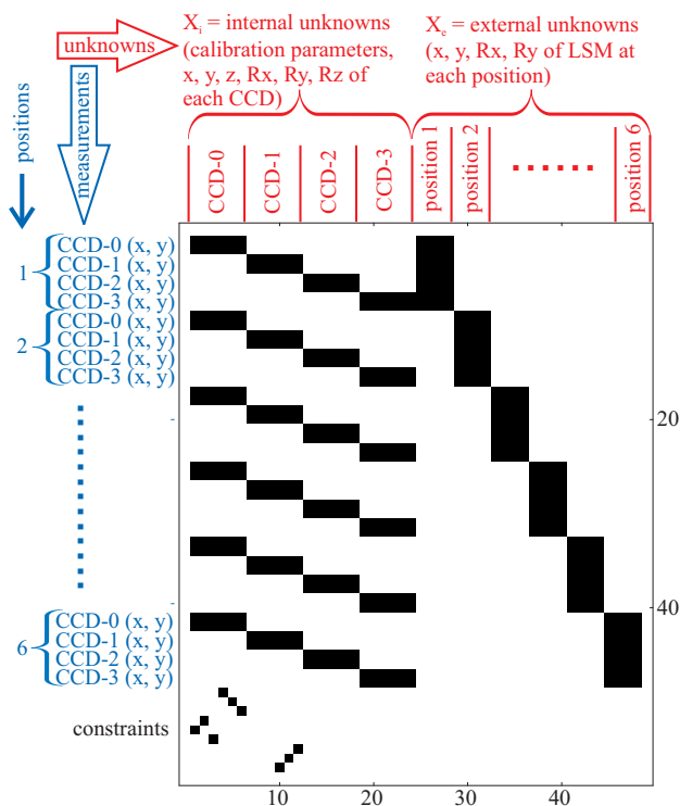
Figure 9: Design Matrix of a six position self calibration process for one LSM unit. Black entries indicate non-zero elements.
