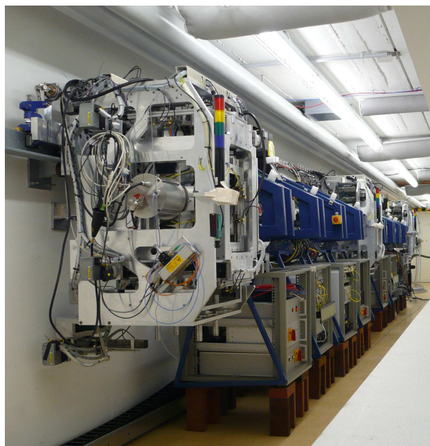
Figure 1: The prototype RTRS after commissioning in the DESY test tunnel (Jan. 2008). The electronics crates in the service cars have temporarily been supported by metal bricks during an analysis of vibration sources.
